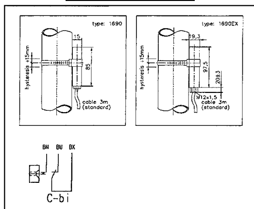
Switch 1690 / 1690ATEX
