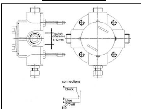
Switch LMS-A-EExd
